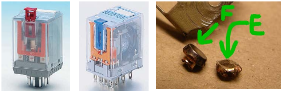
Pic 10, 11 and 12. Industrial relays and contact surfaces. E is the old surface and F is the new.
